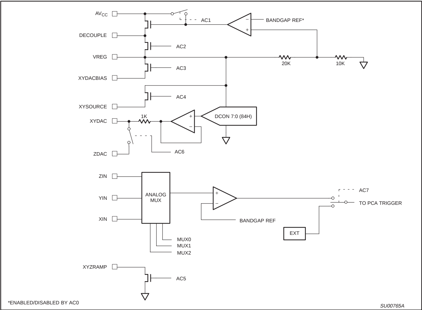
Figure 1. Analog Section
